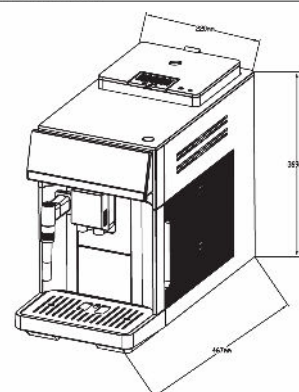
Thermex Coffee - Espresso Plus 1230
