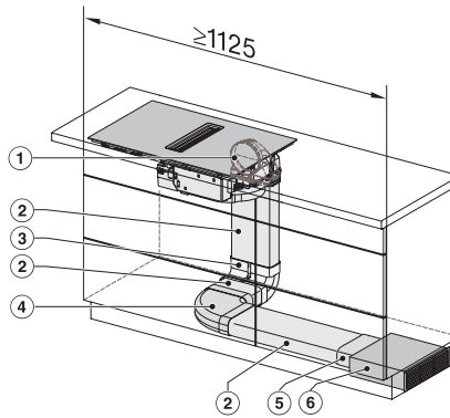
KMDA7272-1FL/FR, KMDA7473-1FL/FL MattFinish/FR, KMDA7272FL/FR, KMDA7473FL/FR – Installation variant 13 Circulating air
