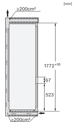
KF7731E, KF7731D, side view
